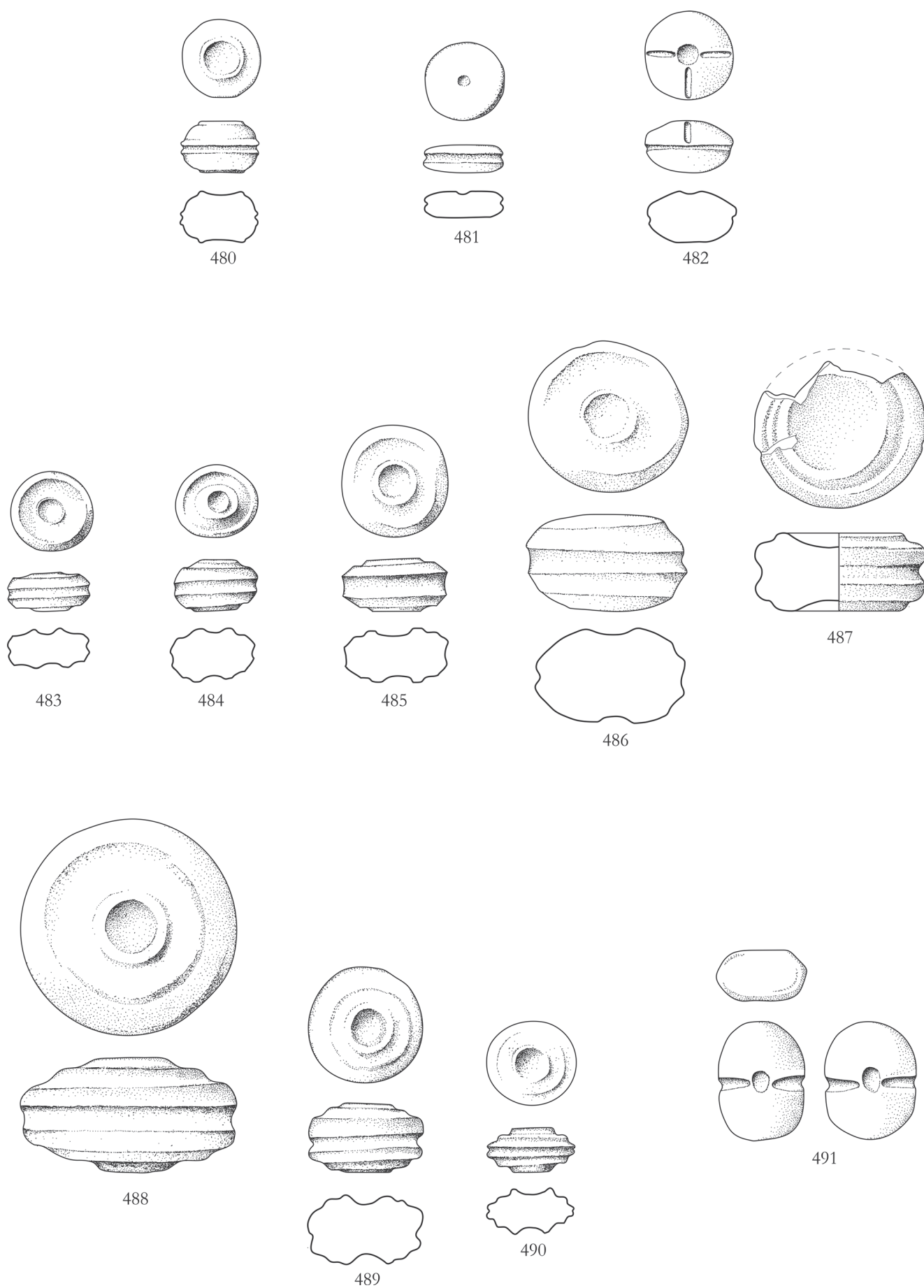
Pl. 28. Kannelurensteine. Variant 2: circular indentations. Sub-variant 2.C: lenticular (cat. no. 480-482). Sub-variant 2.D: multiple horizontal grooves (cat. no. 483-490). Sub-variant 2.E: transversal groove (cat. no. 491). Scale: 1:4.
