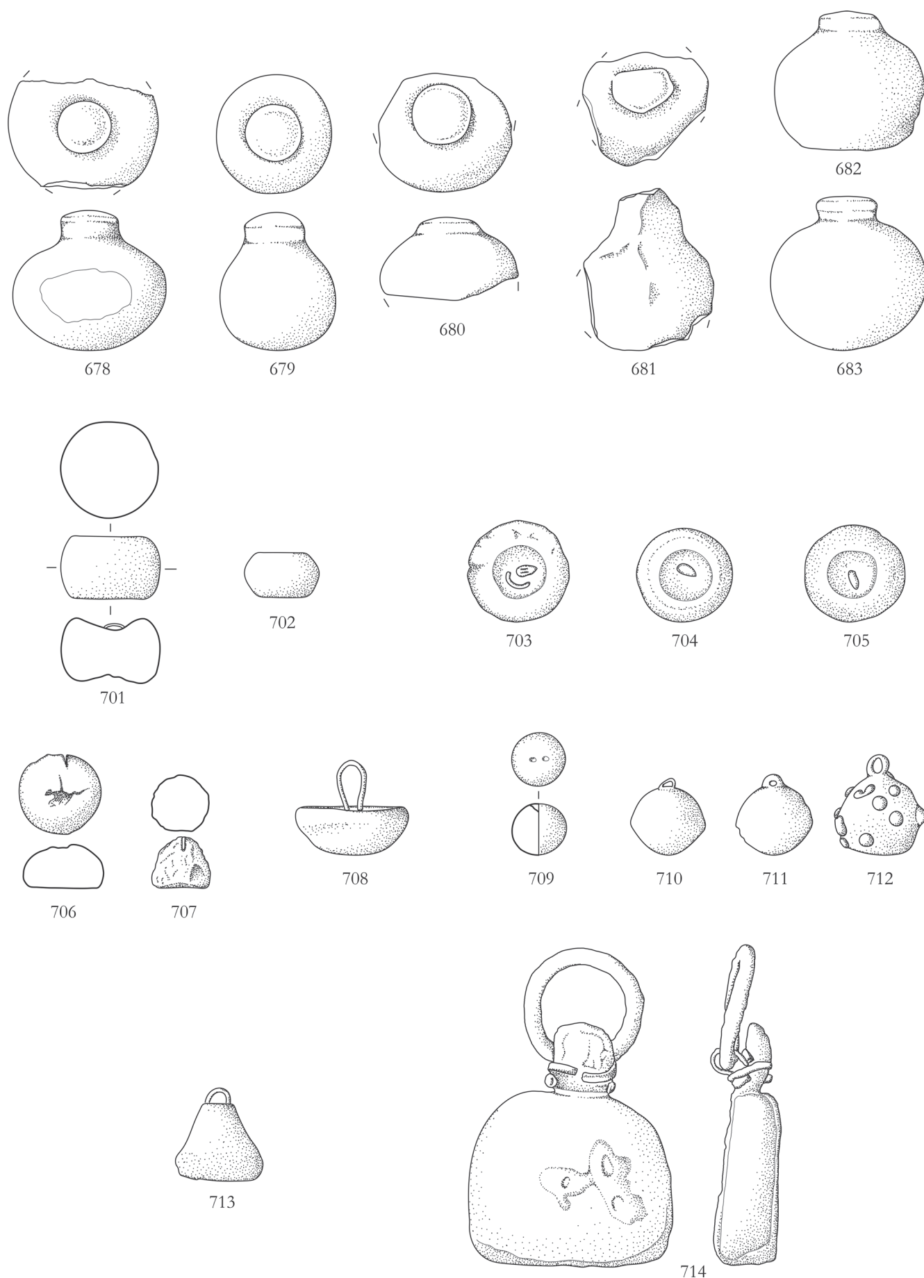
Pl. 31. Piriiform. Variant 2: without perforation. Stone (cat. no. 678-683). Scale: 1:3. Other hanging weights. Variant 1: bi-concave cross-section. Lead (cat. no. 701, 703-705). Stone (cat. no. 702). Variant 2: hemispherical. Lead (cat. no. 706-707). Variant 3: spherical cap. Lead (cat. no. 708). Variant 4: spherical. Stone (cat. no. 709). Lead (cat. no. 710-712). Variant 5: bell-shaped. Lead (cat. no. 713). Variant 6: parallelepiped with upper protrusion. Bronze (cat. no. 714). Scale: 1:4.
