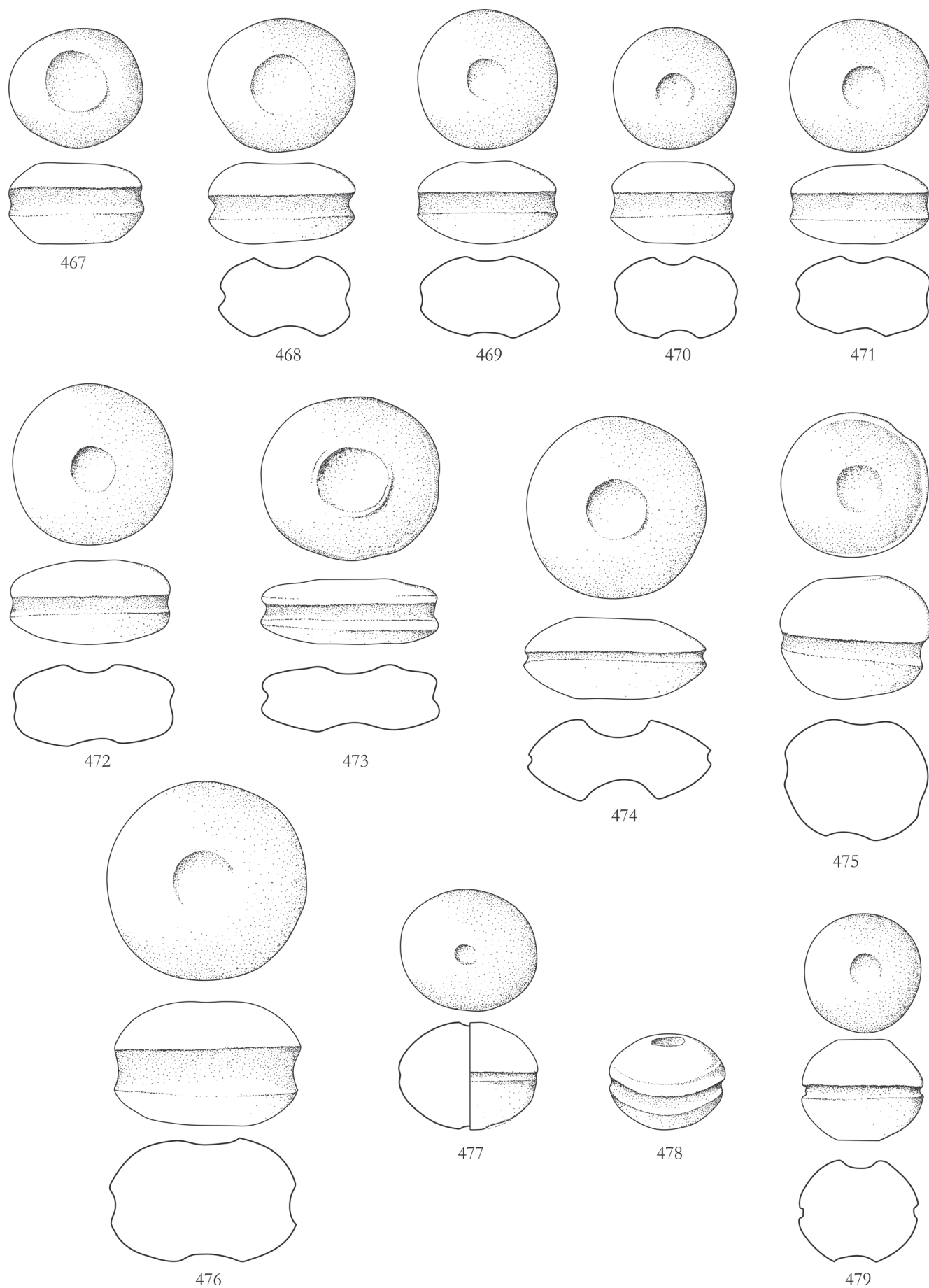
Pl. 27. Kannelurensteine. Variant 2: circular indentations. Sub-variant 2.C: lenticular. Scale: 1:4.
