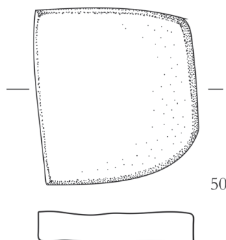
Pl. 3. Parallelepipèd. Variant 1: plain parallelepiped. Stone. Scale: 1:2.
