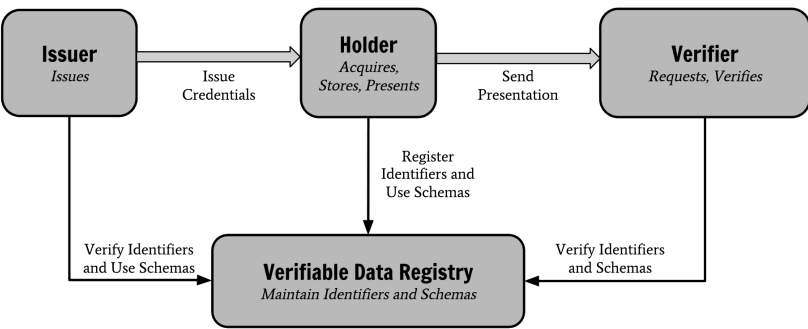
Figure 1. Roles and information flow
