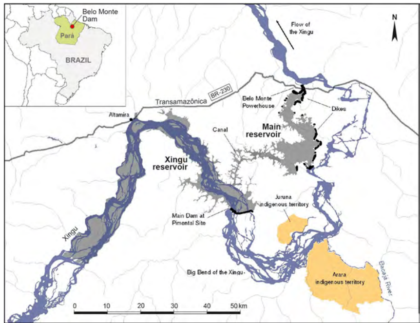
Figure 36. Belo Monte hydro-electric power plant and reservoirs in the Xingu region
