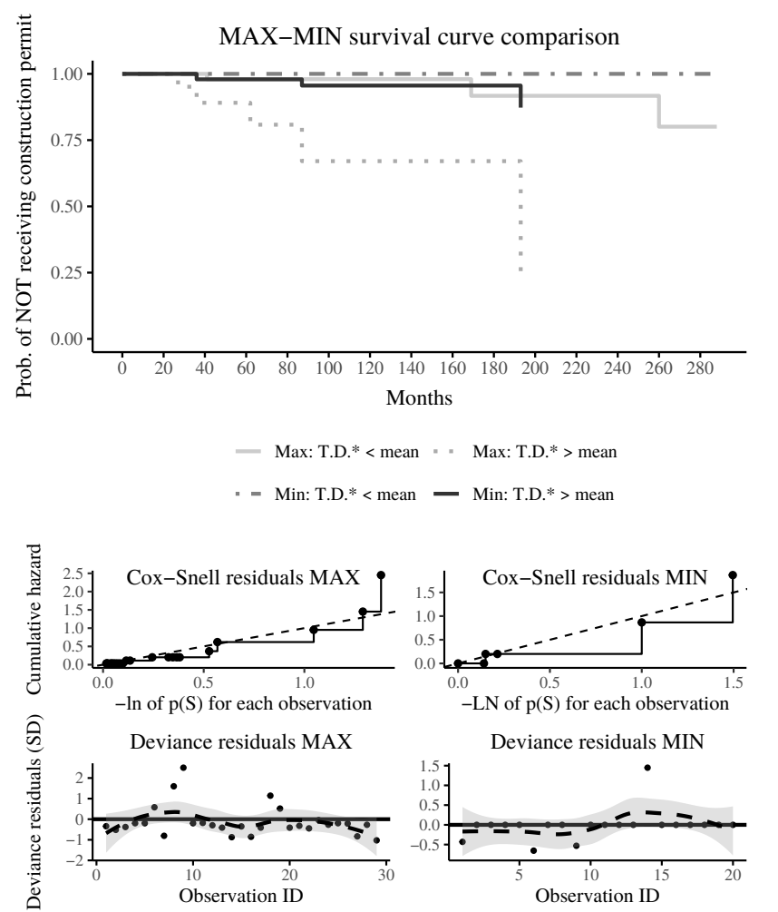
Figure 7.8: Survival curves and model fit graphs for two models with either maximum or minimum effect magnitude of trust density.
