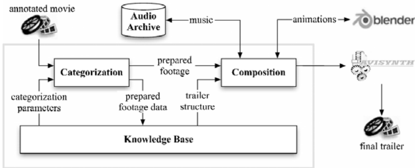
Figure 2: Diagram of the trailer generation process.
