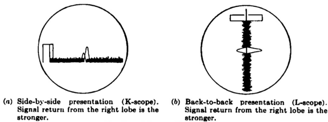
FIG. 6-4.—Pip-matching displays.
