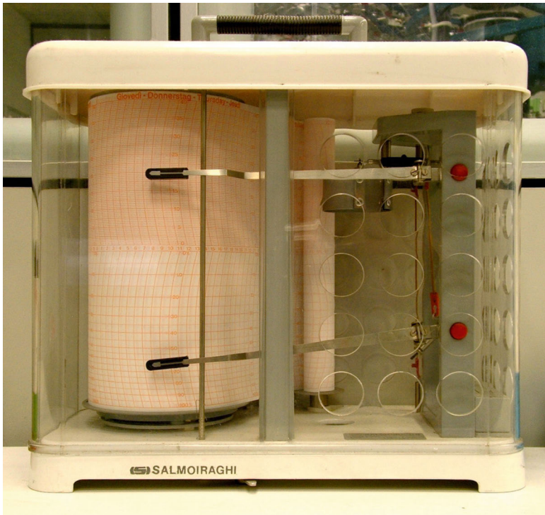
Abb. 2: Hygograph
