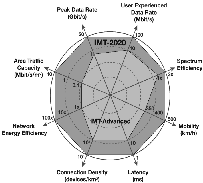
Figure 15: Specification of the technical standard described in the ETSI IMT-2020 documents
