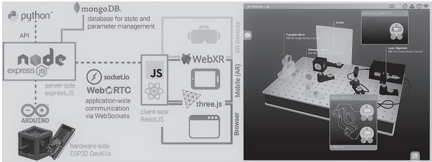
Figure 1: Architecture and Technology Stack with Screenshot of XRTL
