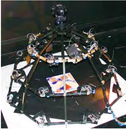
Figure 20.1. Left: experimental apparatus for PTM at the National Gallery (London) with twenty-four tungsten spotlights mounted on a rigid framework. Below: surface relief of a painted test panel, lit from the top right. © Joseph Padfield, National Gallery, London.
