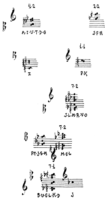
Abb. 41: Cage Song Books Solo 45, Aggregat-Notation (Notationsform VII) 26
