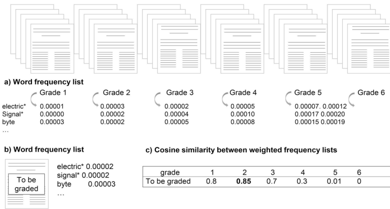
Figure 1: e-rater's grading approach based on word-frequency lists (3 rd number computed in the approach)
