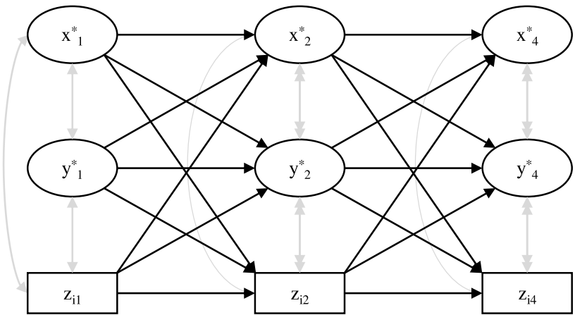
Abbildung 2: Trivariates Crossed-Lagged-Panel-Modell
