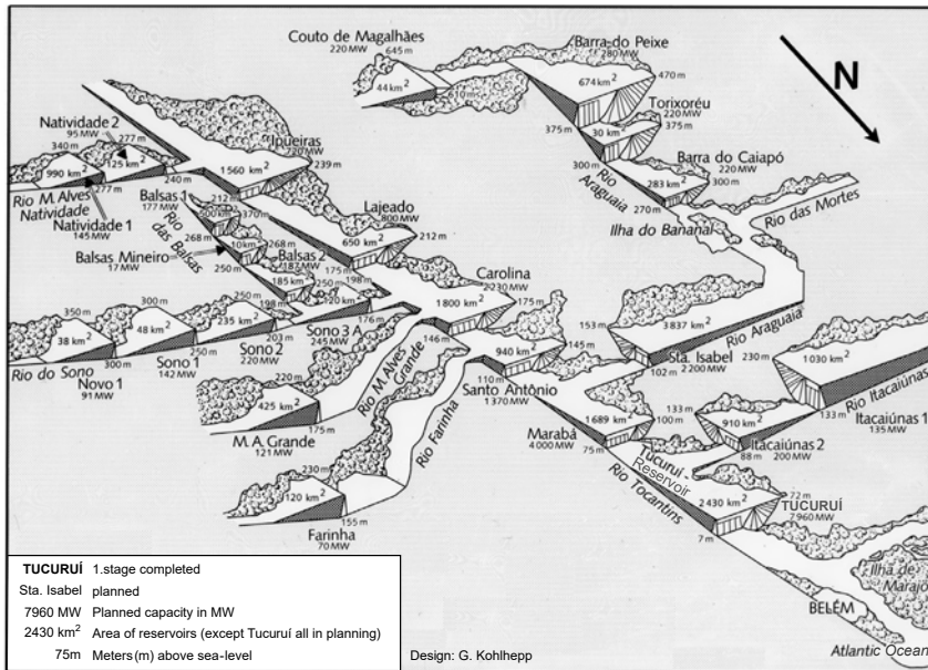
Figure 20. Eletronorte's vision of hydroelectric power plants and reservoirs in the Tocantins-Araguaia river basin
