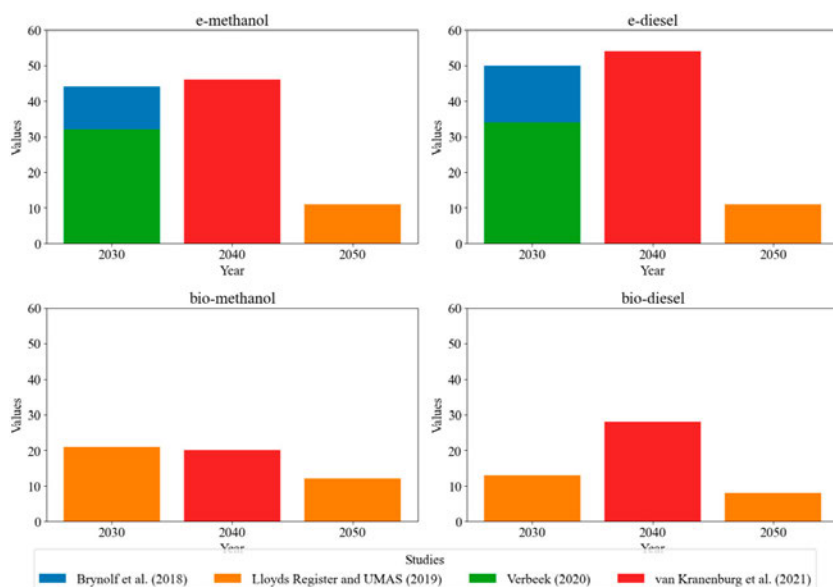
Figure 14.4. E-fuel cost estimates (€/GJ) (Brynnolf, Taljegard, Grahn, & Hansson, 2018; Lloyds Register and UMAS, 2019; Verbeek, 2020; Kranenburg, et al., 2021).
